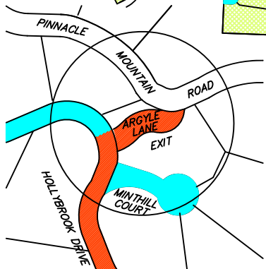
ENLARGED DETAIL OF CONSTRUCTION ENTRANCE/EXIT
